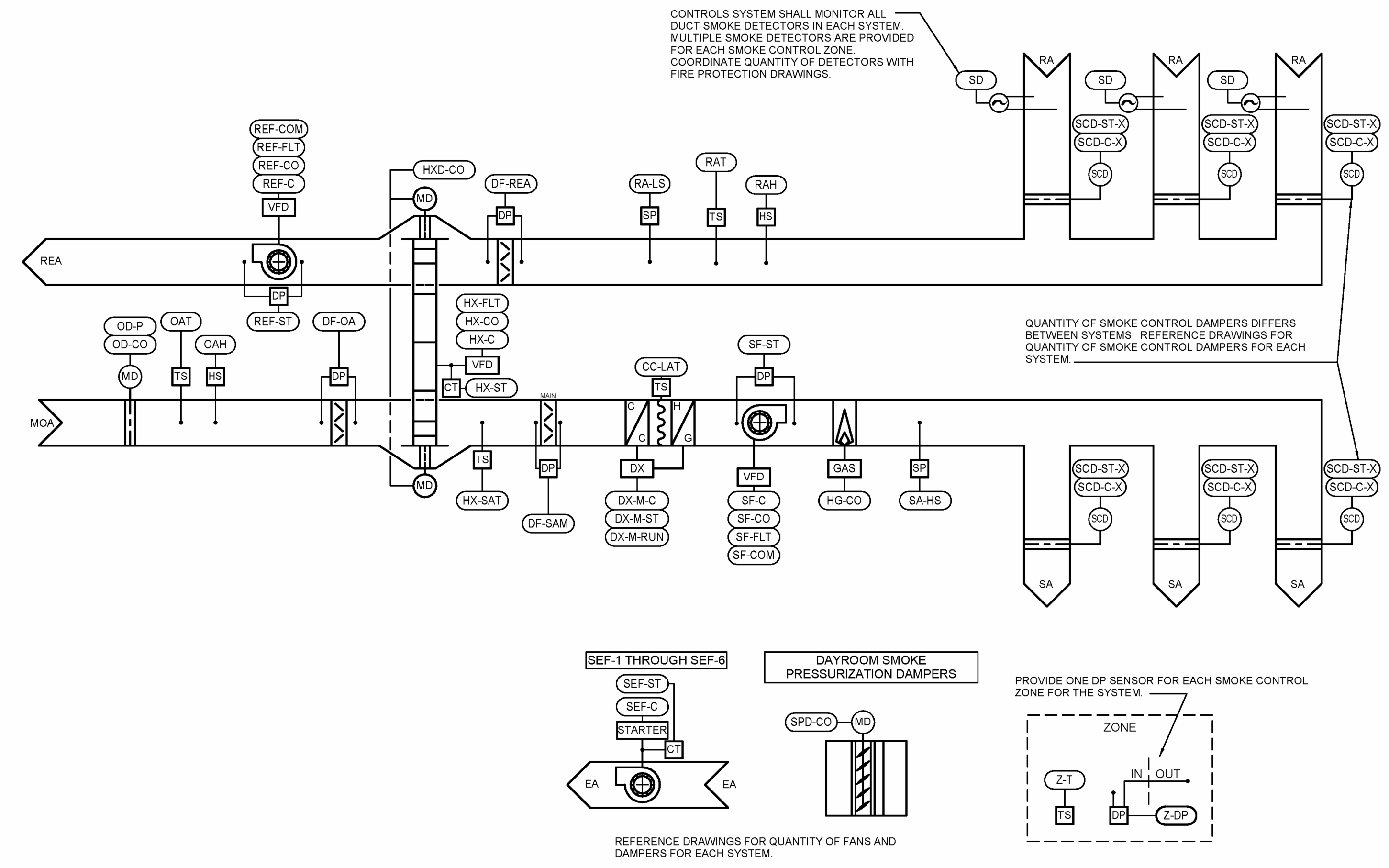
1 RTU-2 AND RTU-3 CONTROL DIAGRAM
