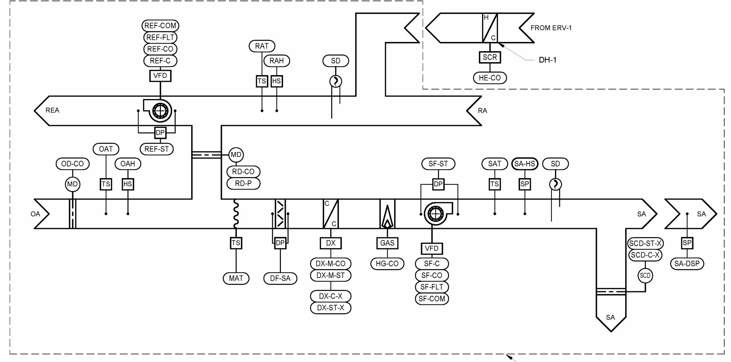
1 RTU-1 & DH-1 CONTROL DIAGRAM NTS
