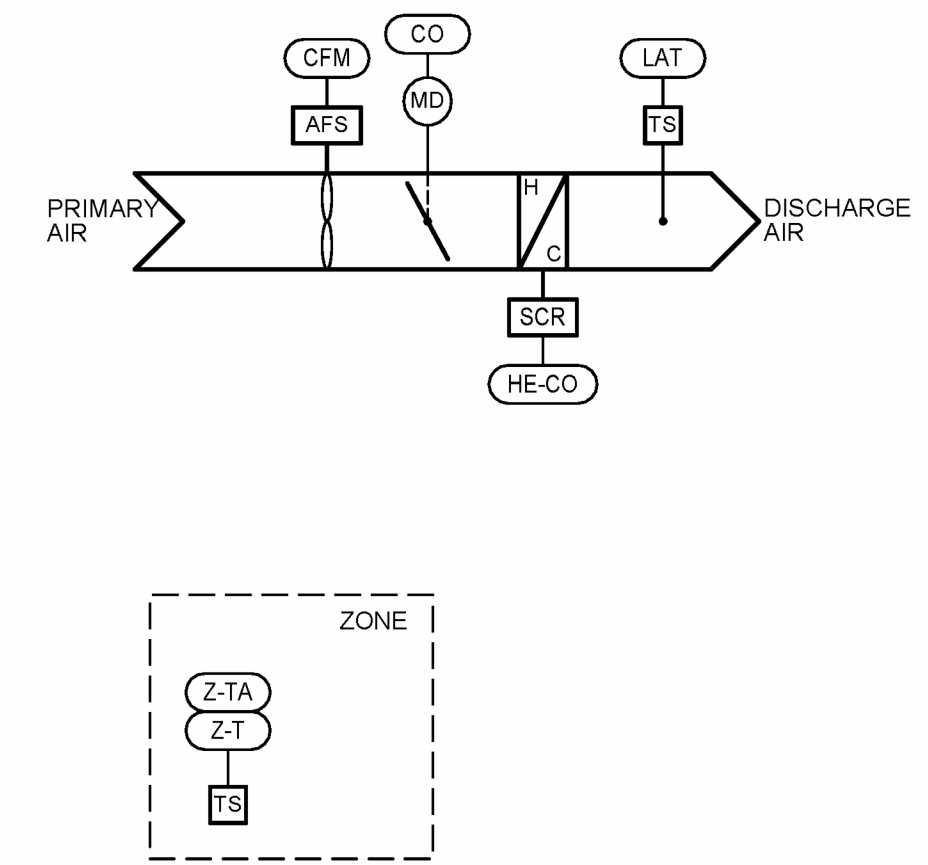
① TERMINAL UNIT CONTROL DIAGRAM 12" = 1'-0"
