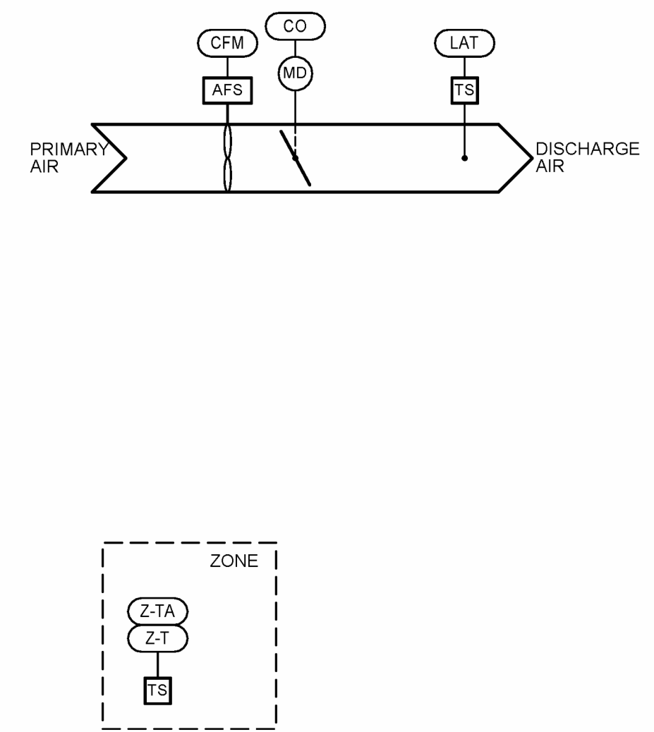
④ TERMINAL UNIT (VAV-1-22) CONTROL DIAGRAM NTS
